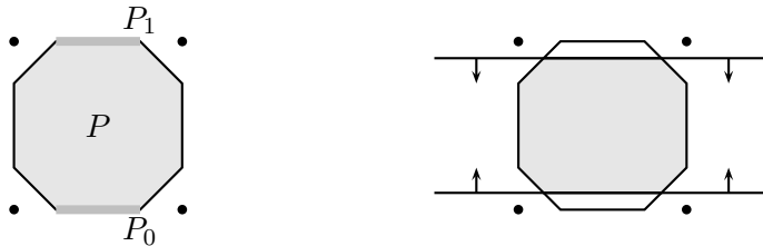
Figure 4.1: After P_0 and P_1 are empty, the Gomory-Chvátal cuts x_n \geq \lceil \epsilon \rceil and x_n \leq \lfloor 1 - \epsilon \rfloor apply for some \epsilon > 0 .
