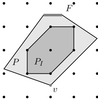
Figure 2.2: This picture illustrates a polyhedron P , one of its vertices v , one of its facets F and its integer hull P_I .
