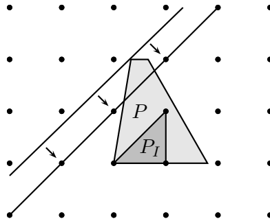
Figure 3.1: The half space (-x_1 + x_2 \leq \delta) containing P is replaced by its integer hull (-x_1 + x_2 \leq \lfloor \delta \rfloor) . The darker region is the integer hull P_I of P .
