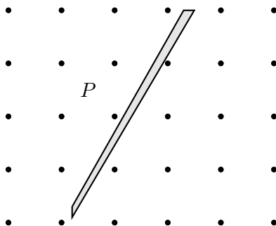
Figure 6.1: A polyhedron P with empty integer hull. P is flat in the direction (-1, 1) .
