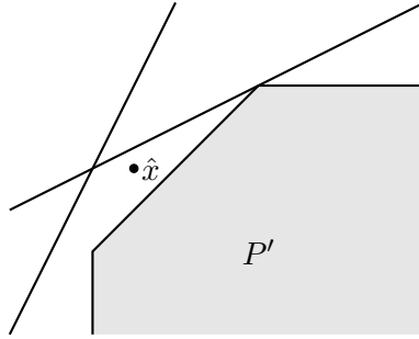
Figure 6.2: The point \hat{x} lies “above” the facet c^T x \leq \delta and “below” each other inequality in (6.10).
