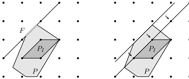
Figure 3.2: After a finite number of iterations F is empty. Then the half space defining F can be pushed further down. This is basically the argument that every inequality, valid for P_I eventually becomes valid for the outcome of the successive application of the elementary closure operation.
